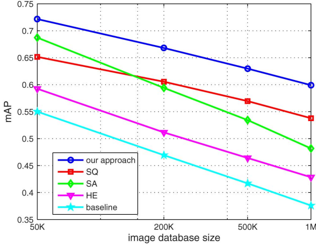
Fig. 9. Comparison of the mAP for 5 approaches on the DuplImage with different numbers of image database images. SQ: scalar quantization [18]; SA: soft assignment [6]; HE: Hamming Embedding [7].
