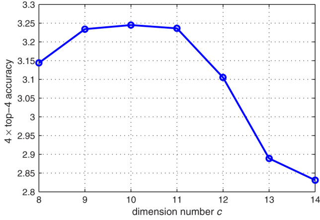
Fig. 7. The performance of the 4 times top-4 accuracy on the UKBench dataset with the 64-bit signature using various values of dimension c , with \tau = 10 and \xi = 0.90 .
