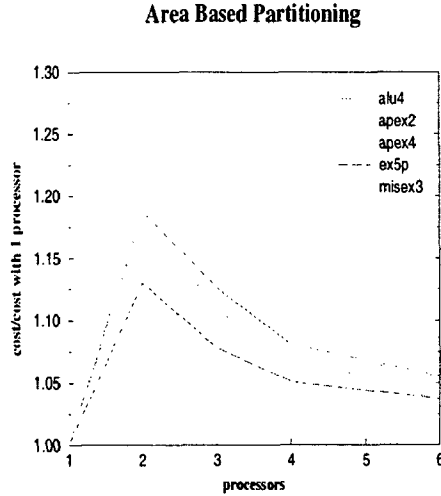
Figure 11: Variation of Normalized Placement Cost for Area based Partitioning algorithm on an SGI shared memory multiprocessor. Cost shown for 1 processor corresponds to the serial algorithm.
