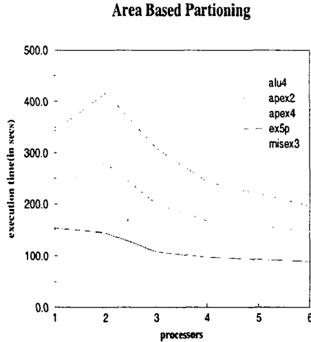
Figure 10: Variation of execution time for Area based Partitioning algorithm on an SGI shared memory multiprocessor. Time shown for 1 processor corresponds to the serial algorithm.
