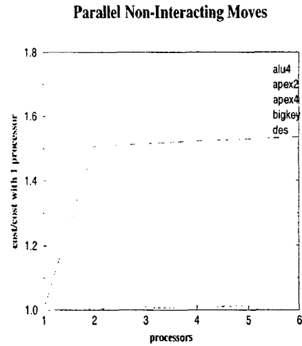
Figure 6: Variation of Normalized Placement Cost for Parallel Moves algorithm on an SGI shared memory multiprocessor. Cost shown for 1 processor corresponds to the serial algorithm.
