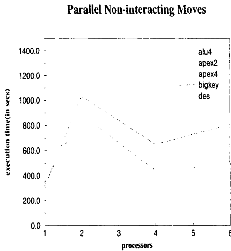
Figure 5: Variation of execution time for Parallel Moves algorithm on an SGI shared memory multiprocessor. Time shown for 1 processor corresponds to the serial algorithm.
