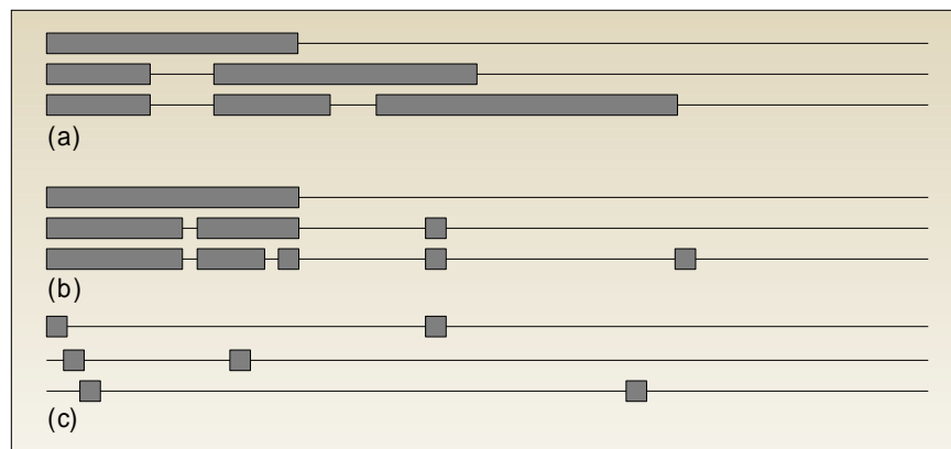
Figure 12. Three alternative methods for training SVMs (a) Chunking, (b) Osuna's algorithm, and (c) SMO. There are three steps for each method. The horizontal thin line at every step represents the training set, while the thick boxes represent the \alpha_i being optimized at that step. A given group of three lines corresponds to three training iterations with the first iteration at the top.
