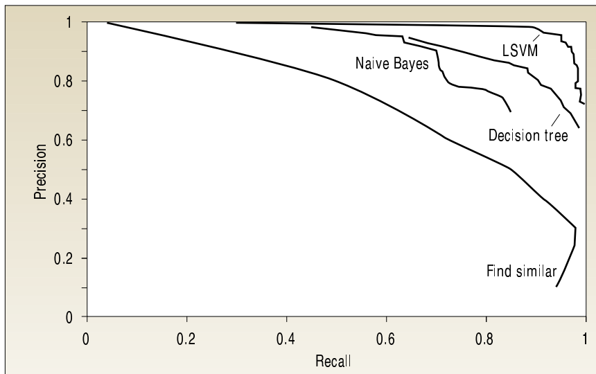
Figure 5. PR curve
