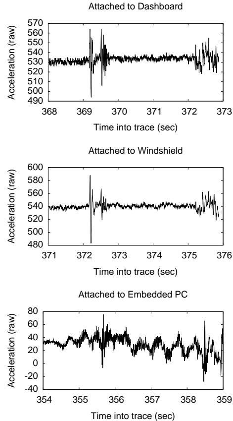
Figure 4: These graphs show the how the accelerometer signal (z axis) varies with placement inside the car. Each graph shows a different placement: either attached to the windshield, dashboard, or attached to the embedded PC. We found firm attachment to the dashboard generated the cleanest signal while still being easy to install.
