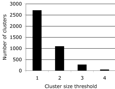
Figure 8: Number of clusters as a function of the cluster size threshold. 48 clusters with 4 or more members were found.
