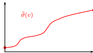
Figure 2: Anti-MHR (e.g., super-exponential): Vickrey is optimal.
