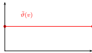
Figure 1: MHR (e.g., uniform): Lottery is optimal.
