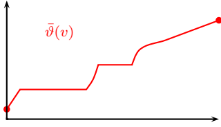
Figure 3: Non-MHR (e.g., bimodal): indirect Vickrey is optimal.
