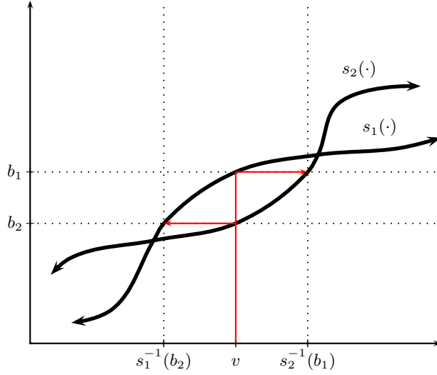
Figure 2.3 Graphical depiction of the first claim in the proof of Lemma 2.15 with b_i = s_i(v) . Clearly, s_2^{-1}(b_1) > s_1^{-1}(b_2) . Strict monotonicity of the distribution function F(\cdot) then implies that F(s_2^{-1}(b_1)) > F(s_1^{-1}(b_2)) .
