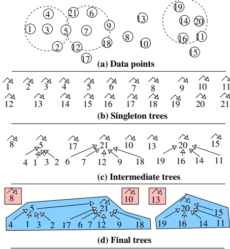
Figure 1. An example showing the proposed DSDBSCAN algorithm at different stages. (a) Sample data points with the circles denoting eps and minpts = 4 . (b) The singleton trees when the algorithm starts. (c) Intermediate trees after exploring the eps -neighborhood of three randomly selected points 3, 7, and 14. (d) The resulting trees when the algorithm terminates where the singleton trees (8, 10, and 13) are noise points and the two blue colored large trees (rooted at 20 and 21) are clusters.
