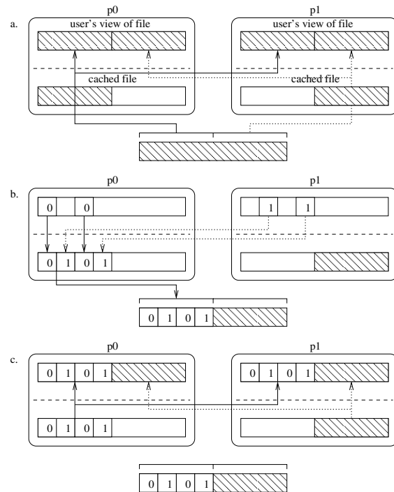
Figure 3. Example file consistency problem solved with persistent file domains.
