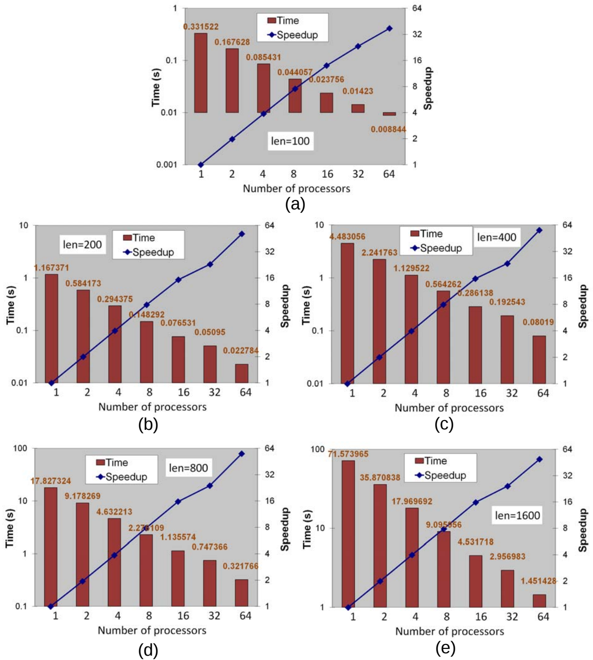
Figure 3: Timing and speed-up results using MPIPairwiseStatSig for sequence-pairs of length (a) 100, (b) 200, (c) 400, (d) 800, (e) 1600.
