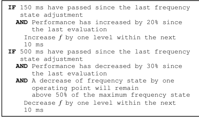
Figure 3. Windows XP DVFS Algorithm
