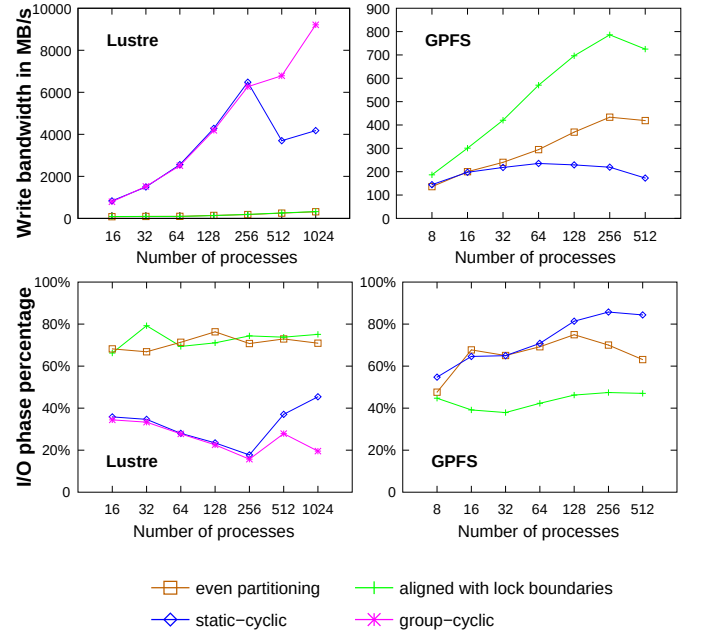
Fig. 12. Performance results for S3D I/O benchmark.
