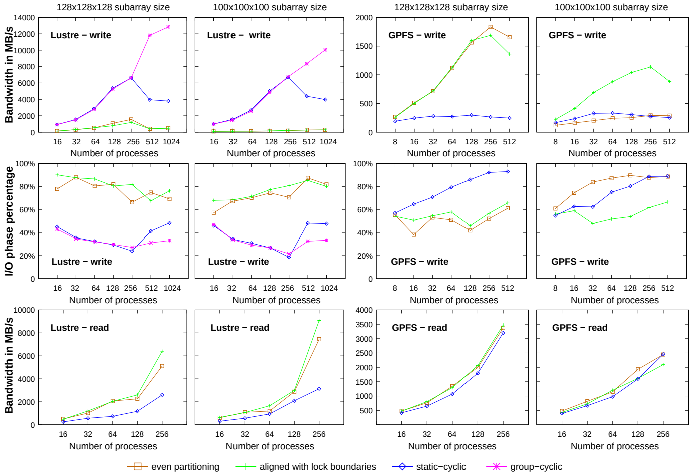
Fig. 6. Performance results of ROMIO collective I/O test.
