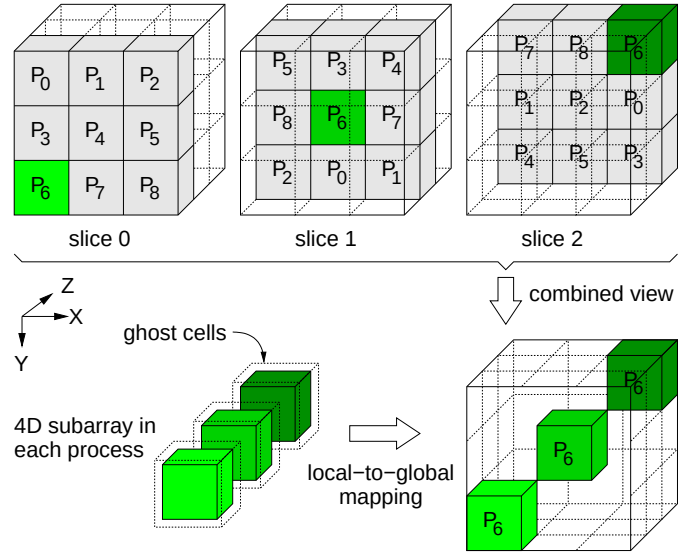
Fig. 7. BTIO data partitioning pattern. The 4D subarray in each process is mapped to the global array in a block-tridiagonal fashion. This example uses 9 processes and highlights the mapping for process P_6 .
