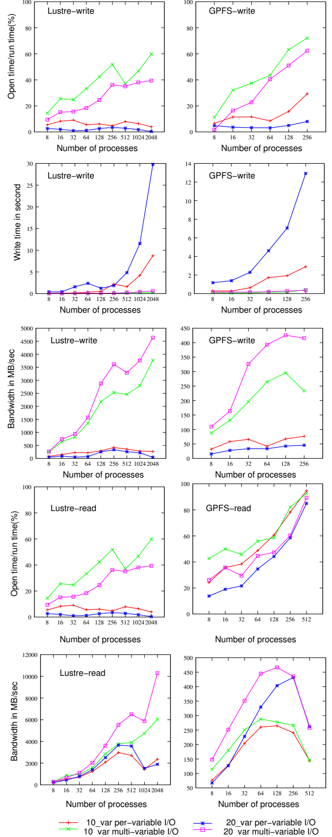
Figure 7. Performance results of ROMIO collective I/O test for record array variables
