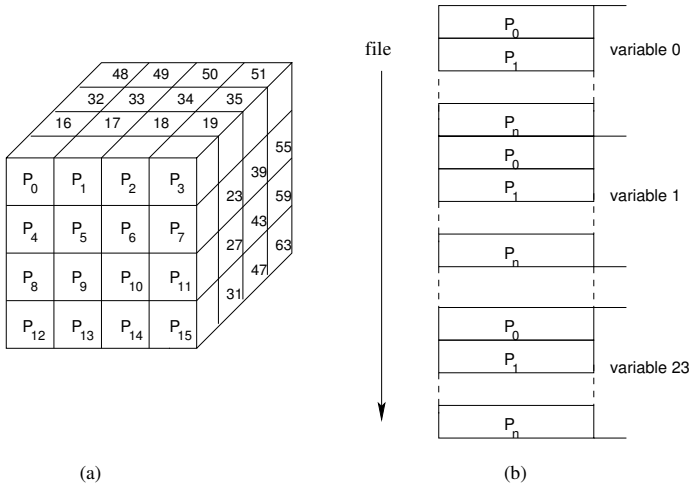
Figure 5. (a) Data partitioning pattern in the ROMIO collective I/O test. A three-dimensional array is partitioned among 64 processes in a block-block fashion. (b) I/O pattern of the FLASH I/O benchmark.
