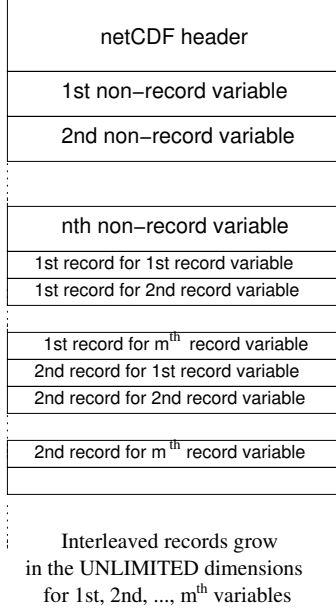
Figure 1. NetCDF file structure
