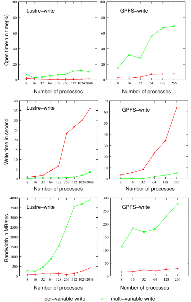
Figure 8. Performance results of FLASH I/O benchmark
