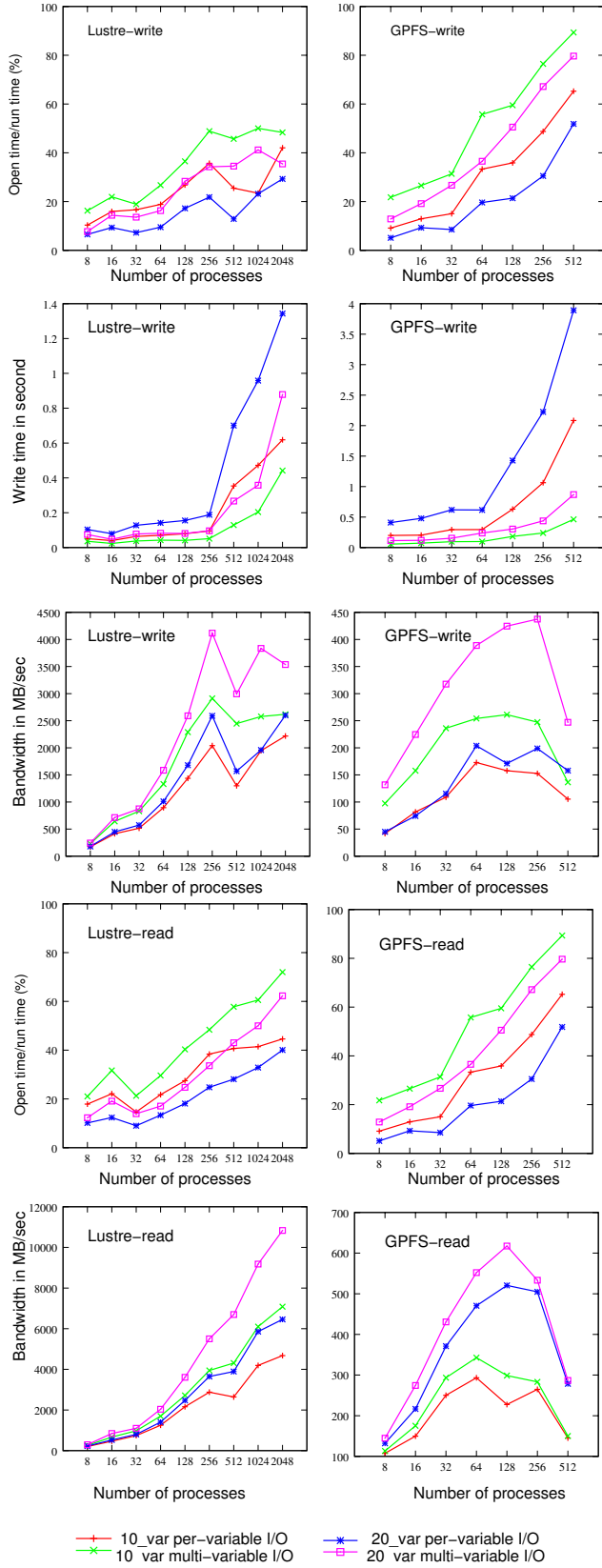
Figure 6. Performance results of ROMIO collective I/O test for non-record array variables
