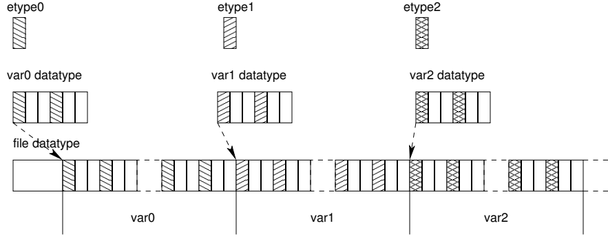
Figure 2. Combining derived datatypes for non-record array variables
