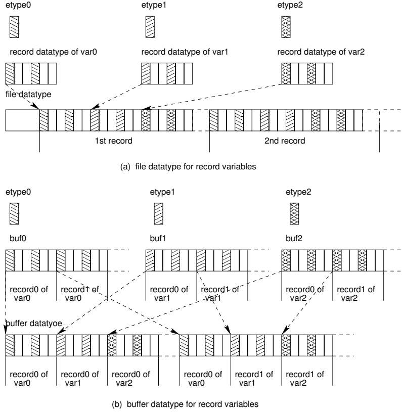
Figure 4. Combining derived datatypes for record array variables
