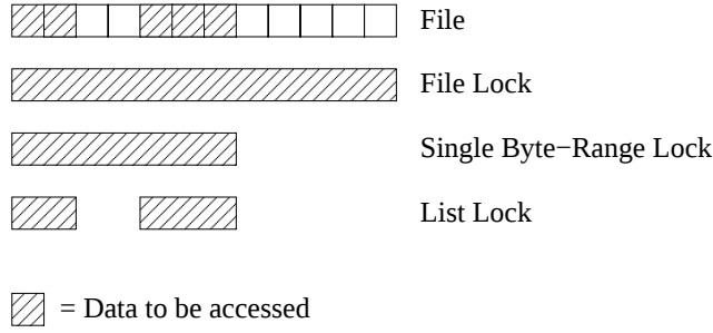
FIGURE 12. A variety of lock-based methods for atomic noncontiguous I/O.
