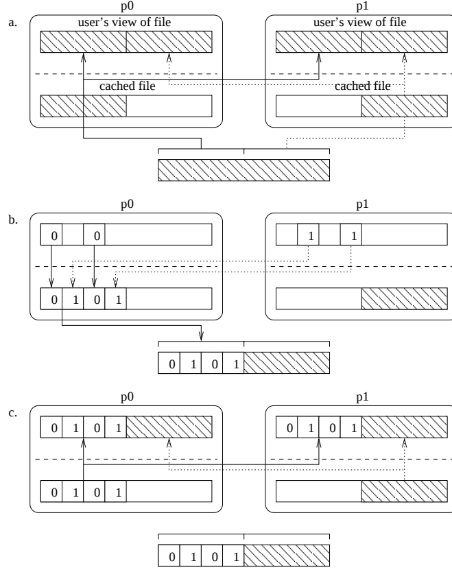
FIGURE 15. Cache consistency issues of collective I/O using persistent file domains.
