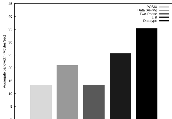
FIGURE 10. Tile display I/O performance.
