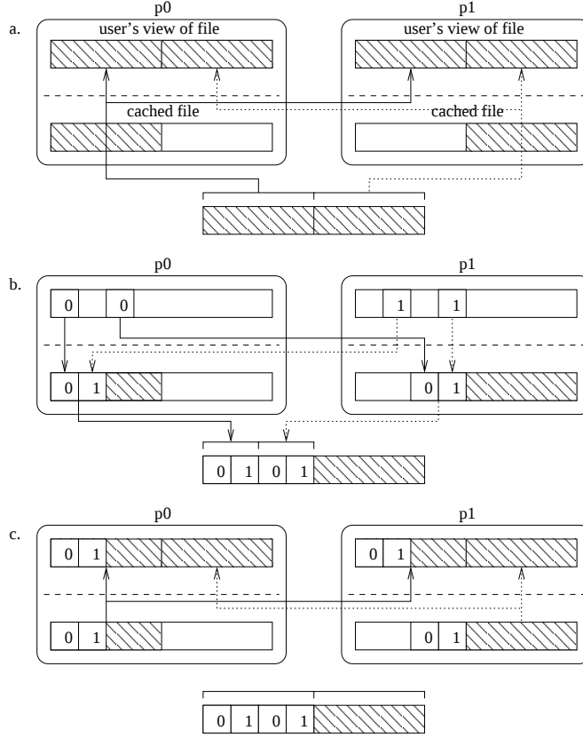
FIGURE 14. Cache inconsistencies in collective I/O
