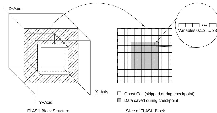
FIGURE 2. ASC FLASH memory block.
