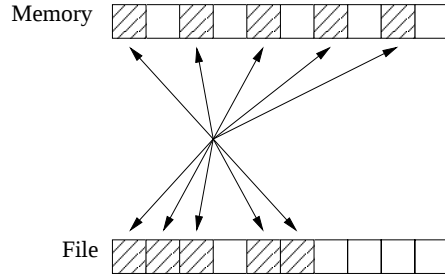
FIGURE 8. Example list I/O call. Only a single I/O request is required to process this noncontiguous access.
