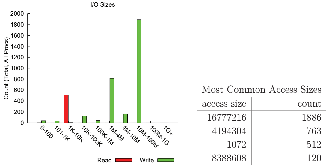
Figure 5. Selected Darshan high-level statistics for the standard file layout. The 512 1072-byte reads should be ignored as they stem from initially reading a configuration file.
