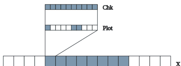
Figure 2. Data extracted from a single block in a 1D simulation with \text{NUNK\_VARS} = 10 (ten mesh variables), \text{nPlotVar} = 3 (three mesh variables for visualization), \text{NXB} = 8 (eight internal cells) and \text{NGUARD} = 4 (four guard cells).
