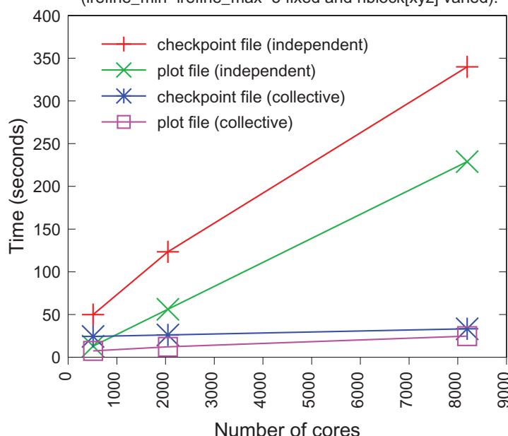
Time for one checkpoint / one plot file during Sedov weak scaling experiments Average of 32 leaf blocks ( 16^3 cells) / process – used HDF5 I/O library (lrefine_min=lrefine_max=5 fixed and nblock[xyz] varied).
