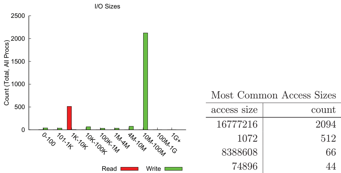
Figure 6. Selected Darshan high-level statistics for experimental file layout. The 512 1072-byte reads should be ignored as they stem from initially reading a configuration file.
