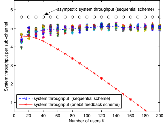
Fig. 6. Achievable rate per sub-channel for the sequential scheme as a function of K for \rho = 1 . Also shown is the achievable rate for the one-bit feedback scheme presented in [5]
