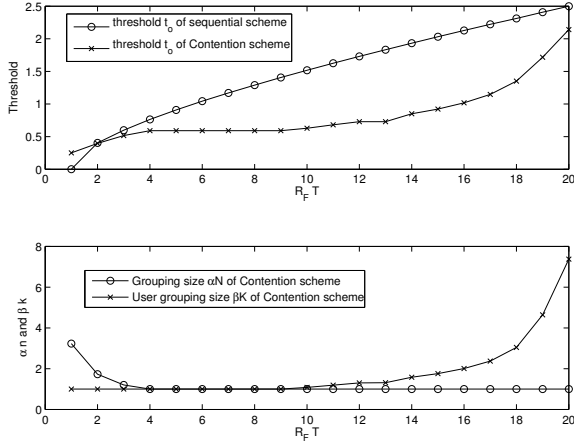
Fig. 4. Optimized parameters for each feedback scheme versus R_F T .
