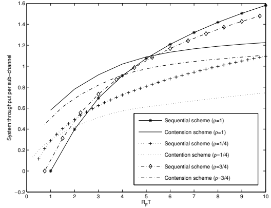
Fig. 2. Asymptotic capacity per sub-channel versus feedback R_F T for the sequential and contention feedback schemes with different loads \rho .
