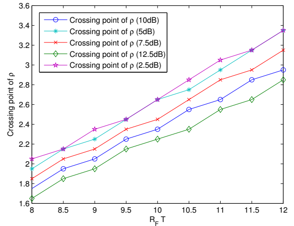
Fig. 3. The crossing point \rho^* as a function of R_F T .
