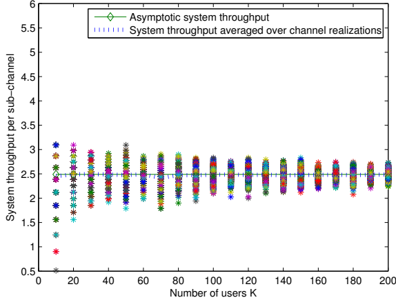
Fig. 5. Achievable rate per sub-channel for the contention scheme as a function of K for \rho = 1 . Each point corresponds to a different channel realization.
